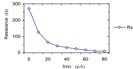
Fig.1 Resistance Rx as a function of IDN3 (9pt Bold, Italic, Times)
